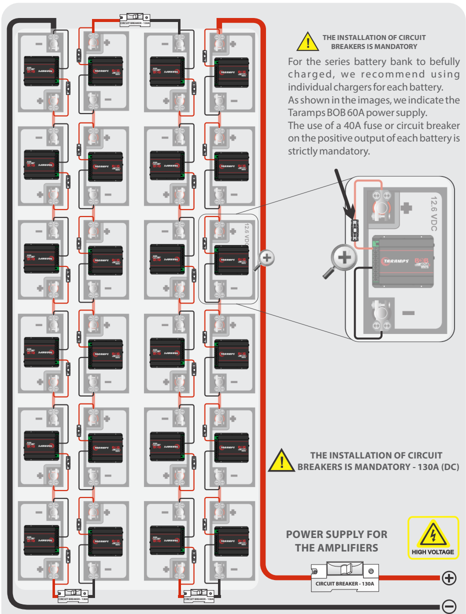
Example of series connection - 24 batteries of 12.6VDC
