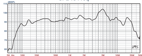
SPL vs Freq
