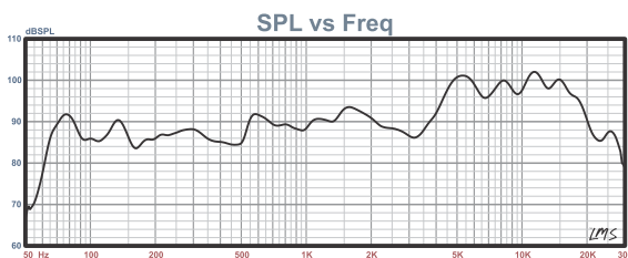
Response curve obtained in a 15L x 75Hz box - (1W x 1m). Response: 65Hz to 27kHz (-6 dB) Average reference 92 dB SPL
