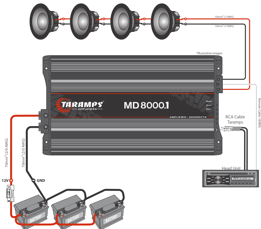
Examples of connections in the power supply input. Note: Required battery bank capacity: At least 370Ah
